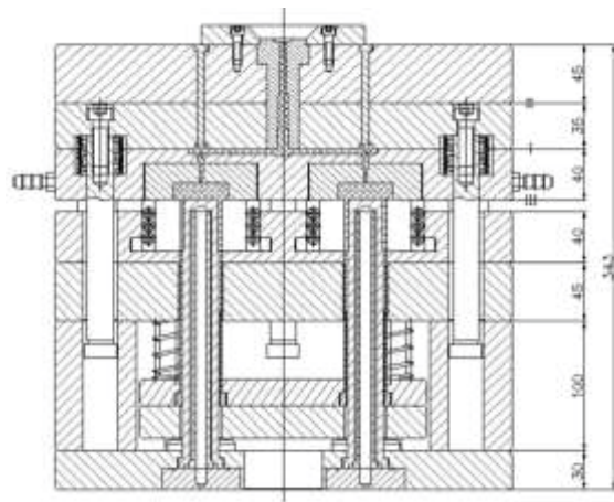
DESIGN OF A FIXTURE
